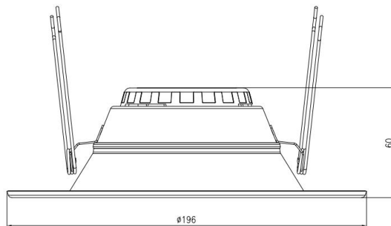
Size : Φ196x60mm(7.72x2.36")
