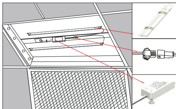
4. Install LED Magnetic strips
