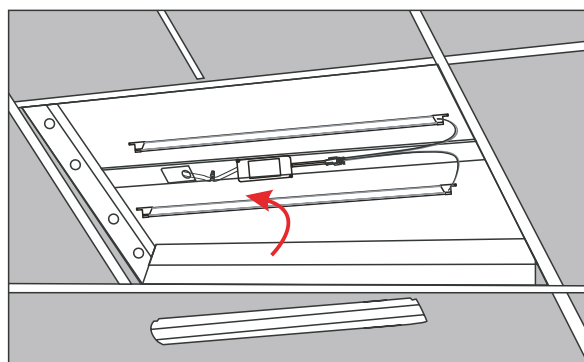
6. Install the Reflector
